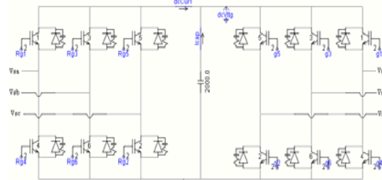
Fig. 3 Circuit of UPFC using IGBTs
