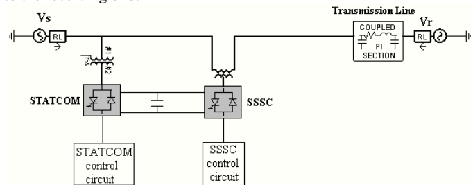
Fig. 2 Power system study model
