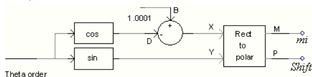
Fig. 6 Series inverter open loop phase angle controller
