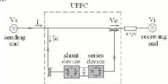
Fig.1 Basic functional scheme of UPFC
