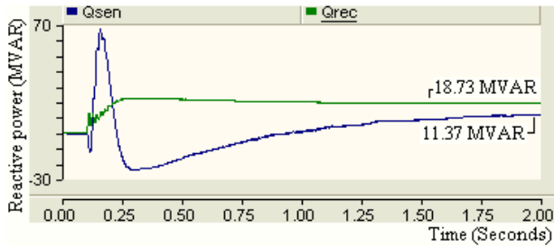
Fig.9 Sending end and receiving end reactive power (a) Without UPFC (b) With UPFC
