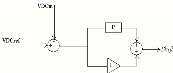
Fig. 4 STATCOM DC voltage controller
